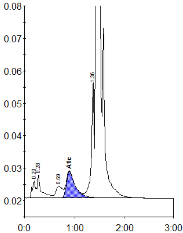
Peak table - ID: 10571747
